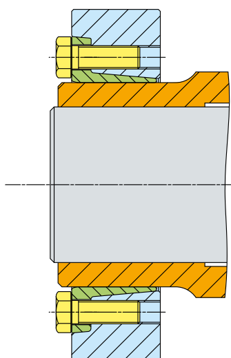
IDC 1700 & 2100: the two flanges create a single block and guarantee the perfect parallel setting after the screw tightening
