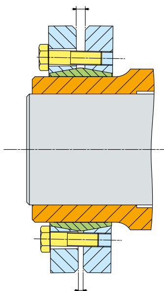
Traditional IDC S100: fitting the two flanges does not guarantee their parallel setting
