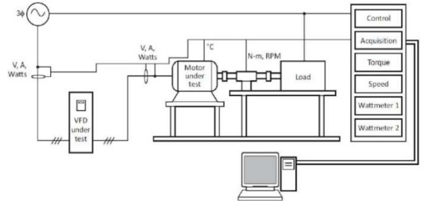
Figure 1 Test Bench and Measurement System Set-up
