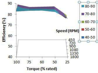
Figure 6 System Efficiency IM-ASD
